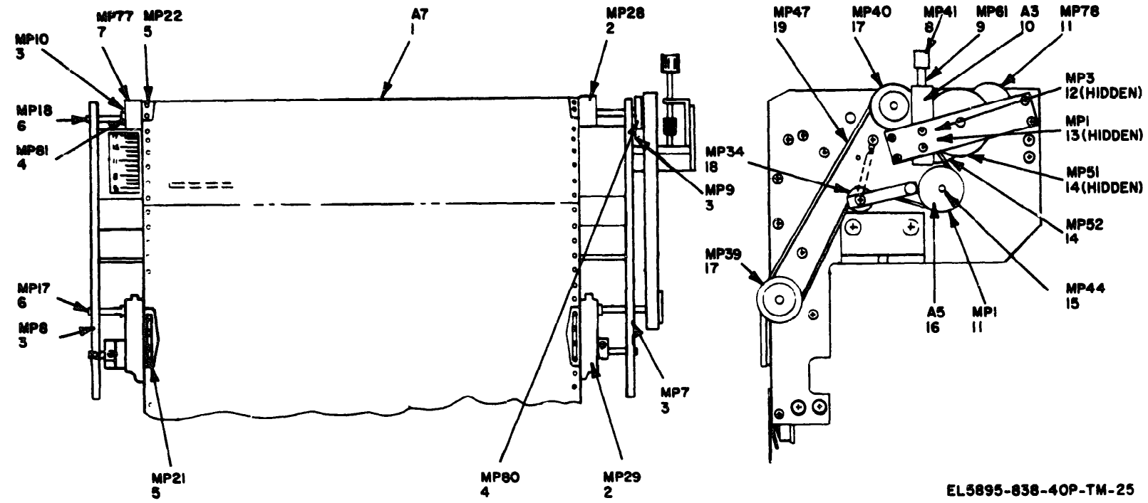
Figure 25. Paper feed mechanism 44548 11 parts location
