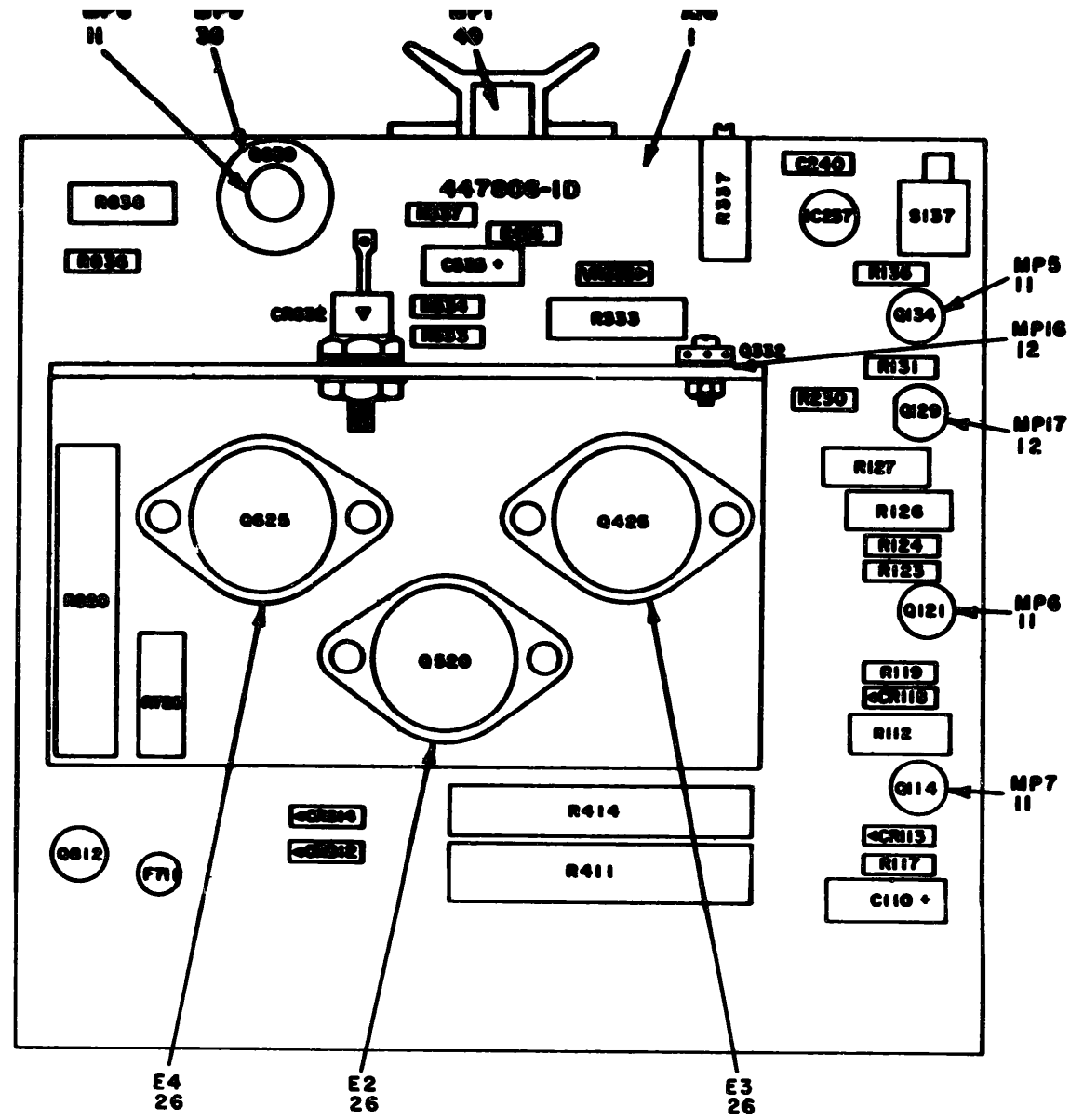
Figure 21. Circuit card assembly, 447806-001D (high voltage control), parts location
