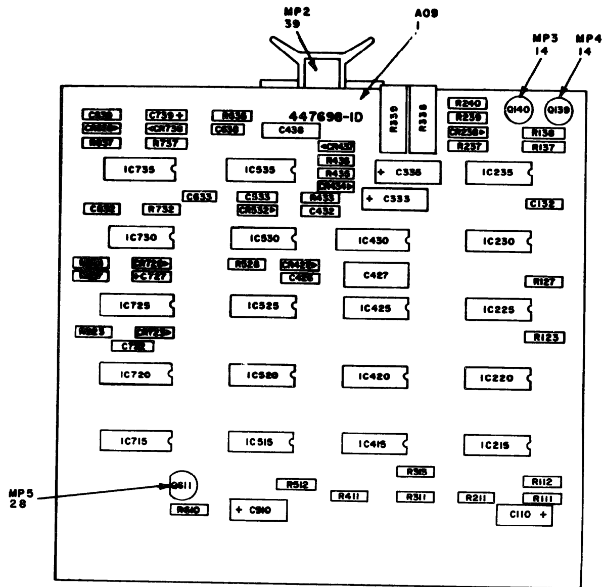
Figure 18 . Circuit card assembly, 447698-001E (paper oscillator and helix control), parts location
