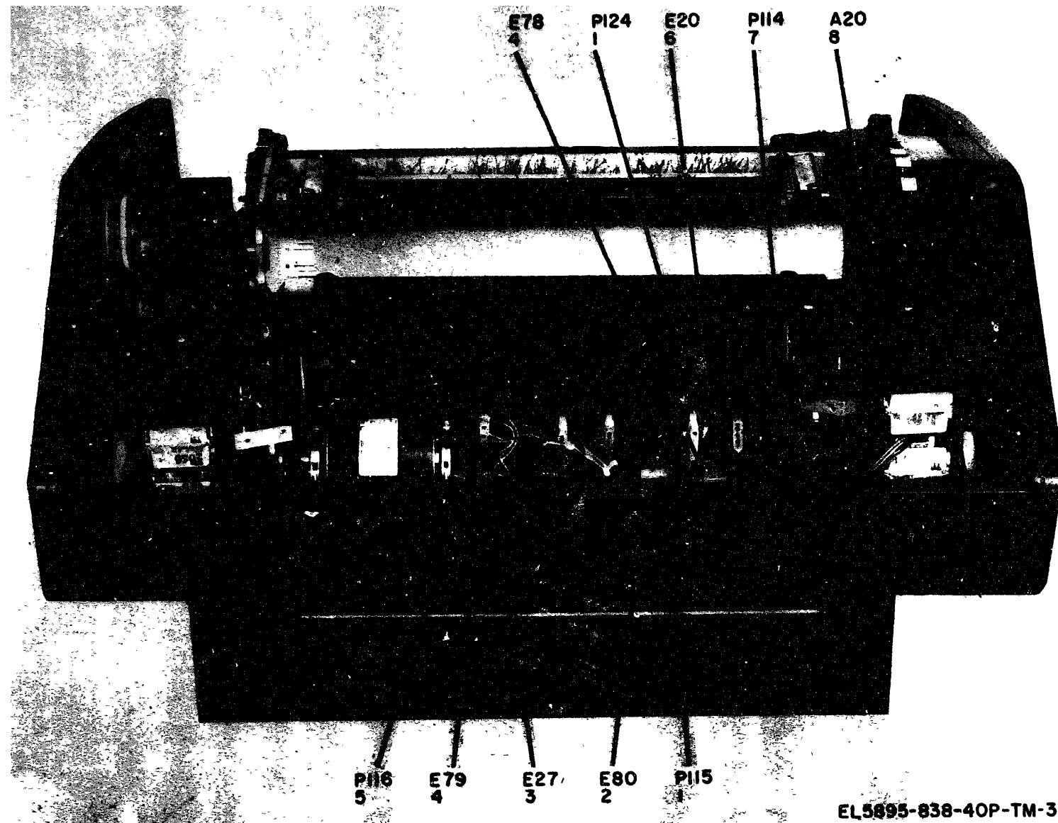
Figure 3. Line printer, top front view, parts location
