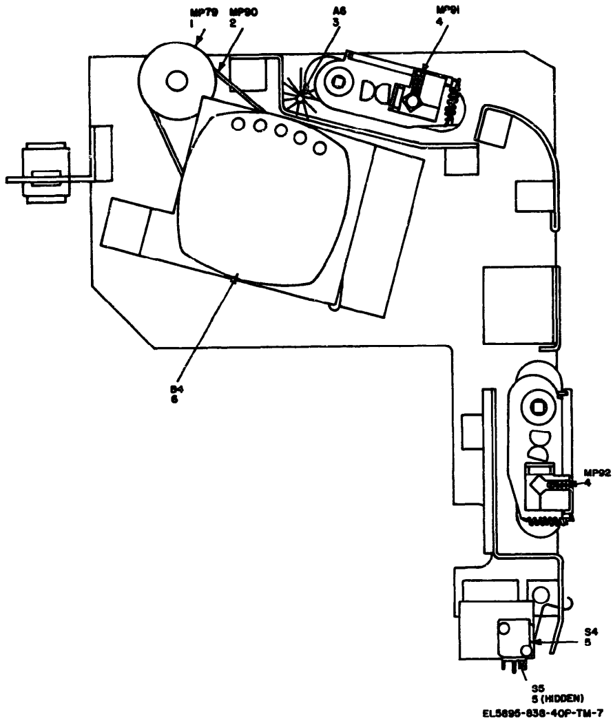
Figure 7. Printer subassembly, 445400-1AJ. side view parts location
