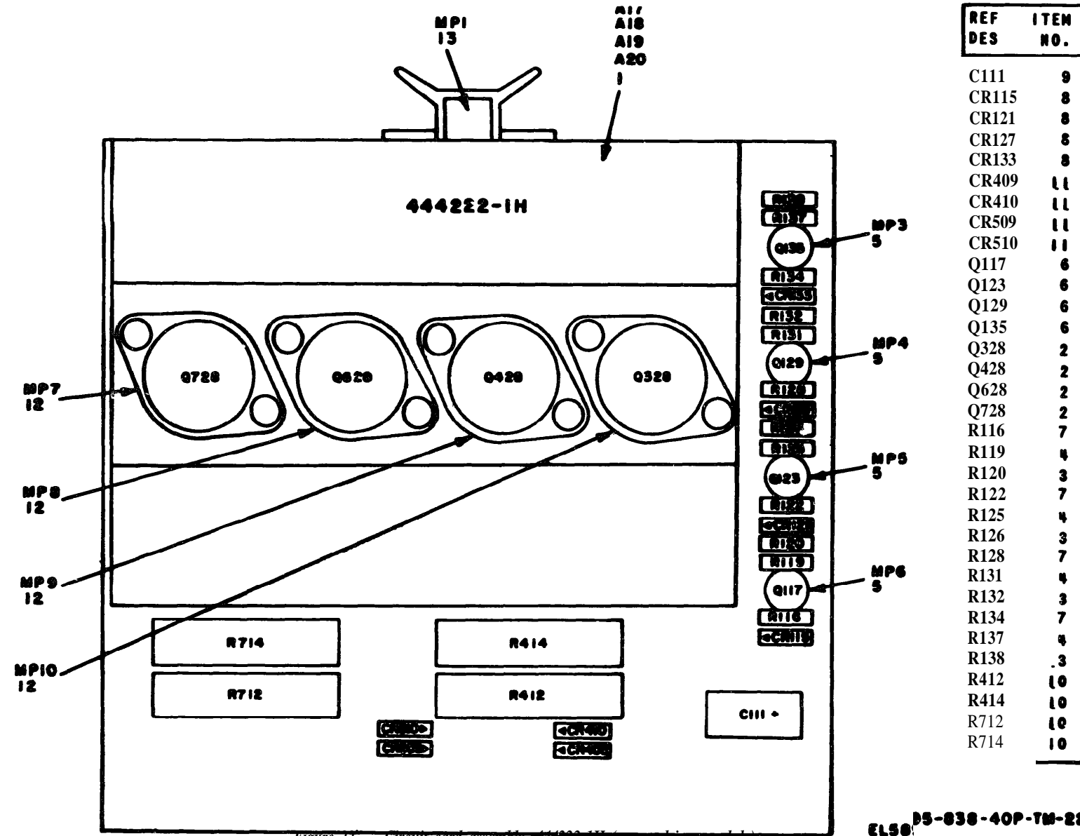
Figure 22 . Circuit card assembly, 444222-1H (power driver module), parts location
