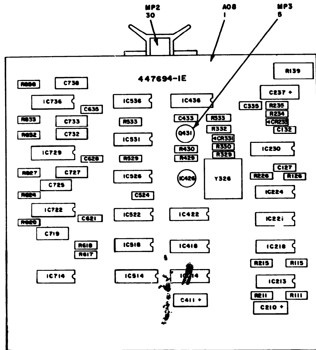
Figure 17. Circuit card assembly. 447694-1E (timing control), parts location
