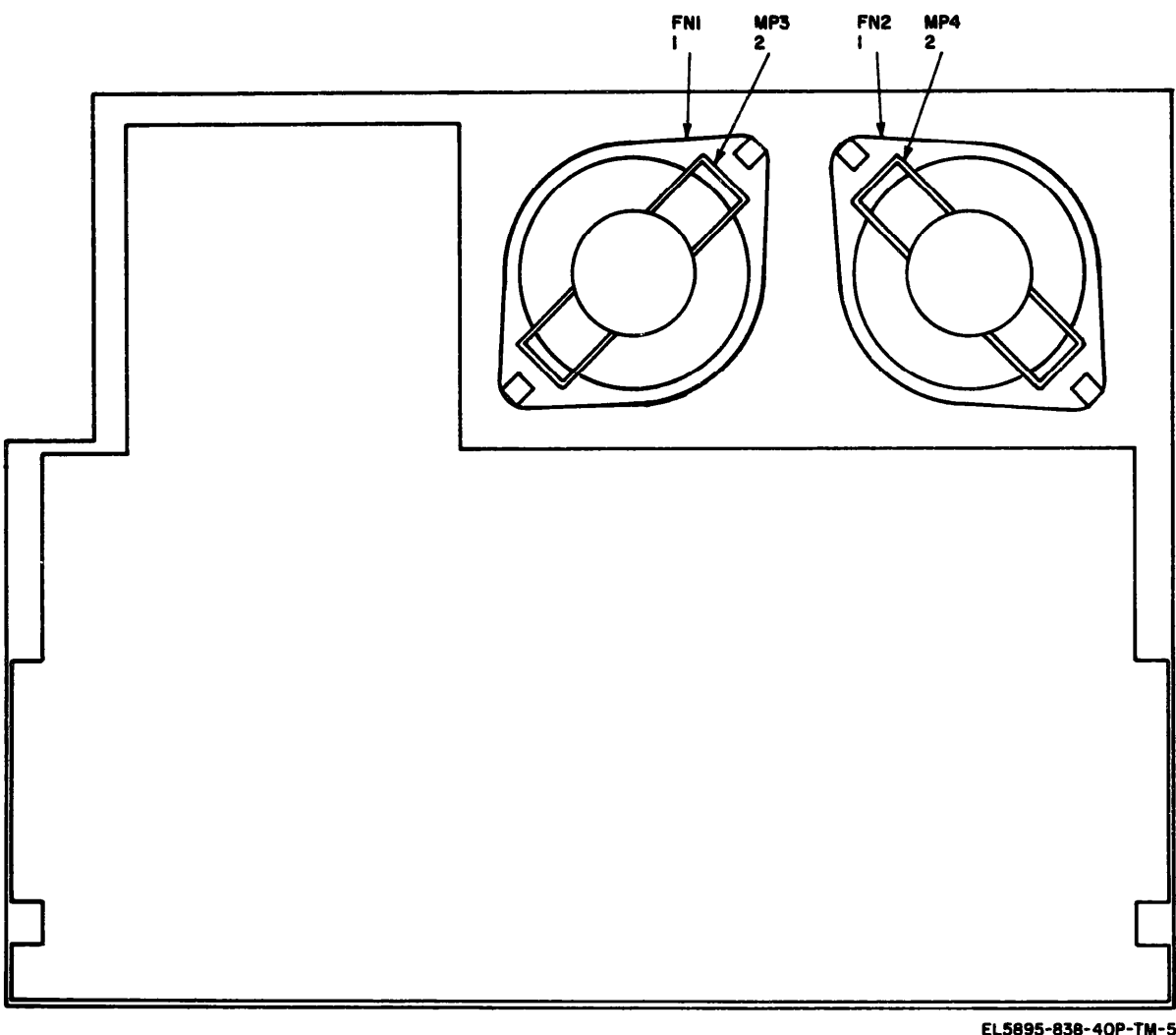
Figure 5 Line printer. bottom view of fan parts location
