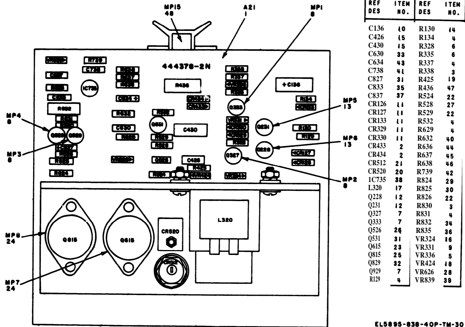
Figure 23. Circuit card assembly, 444378-002N ( \pm 5 volt regulator), parts location
