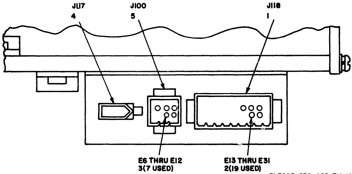
Figure 11. Printer subassembly, 445400-1AJ contact and connector. parts location
