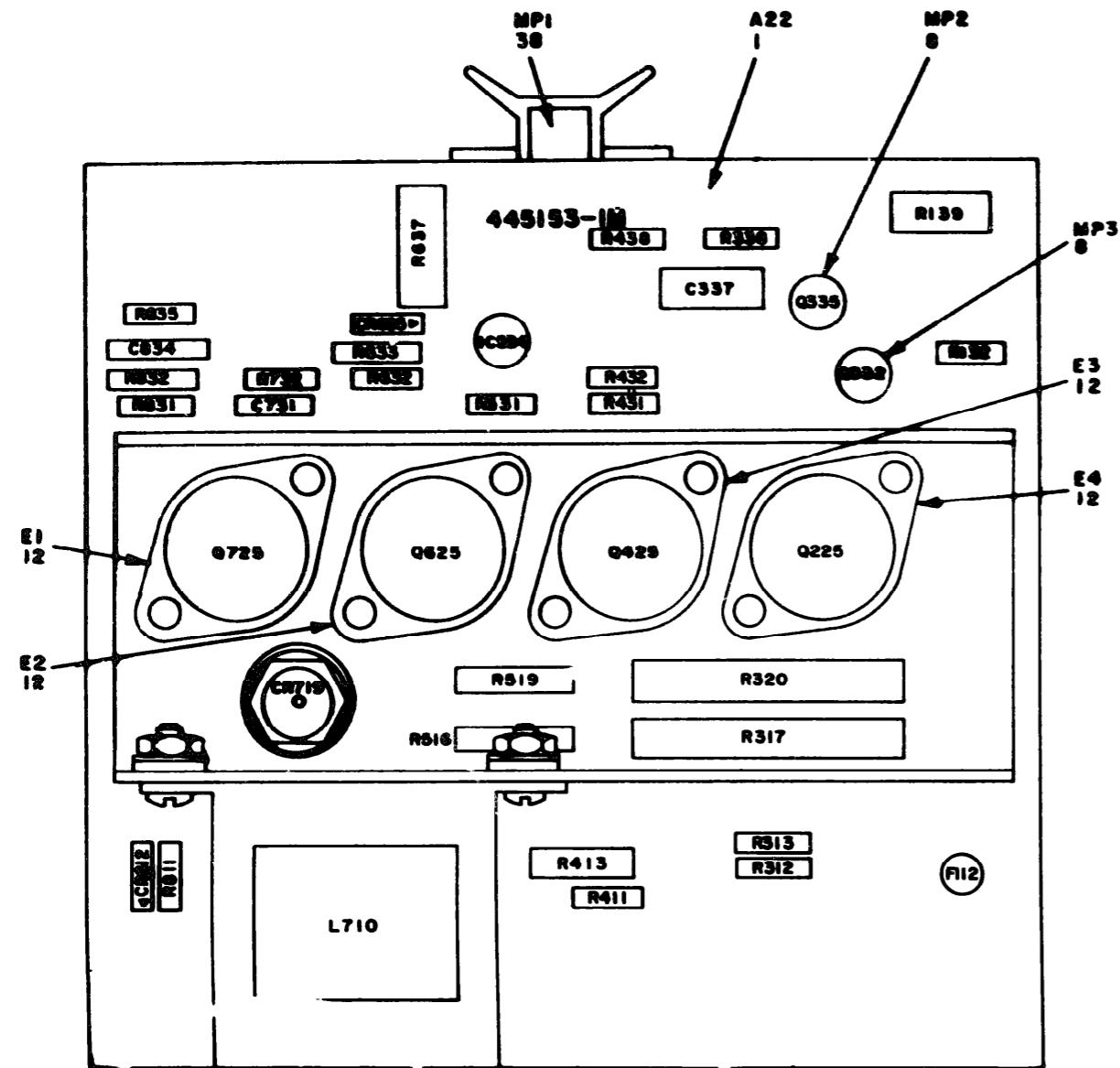
Figure 24. Circuit card assembly 445153-001M (±28 volt regulator), parts location
