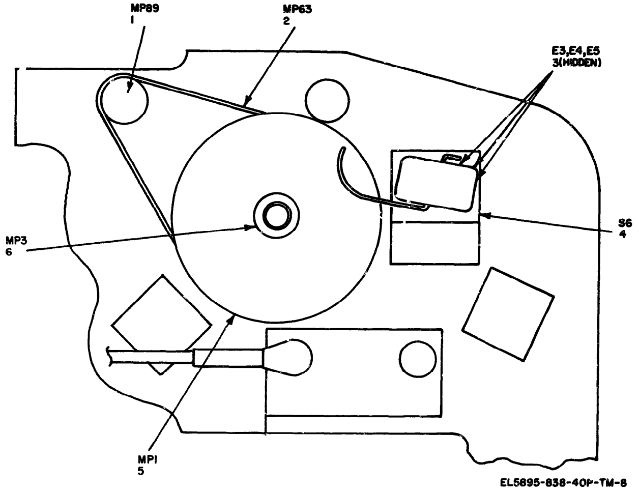
Figure 8. Printer subassembly 445400-1AJ pulley assembly, side view, parts location
