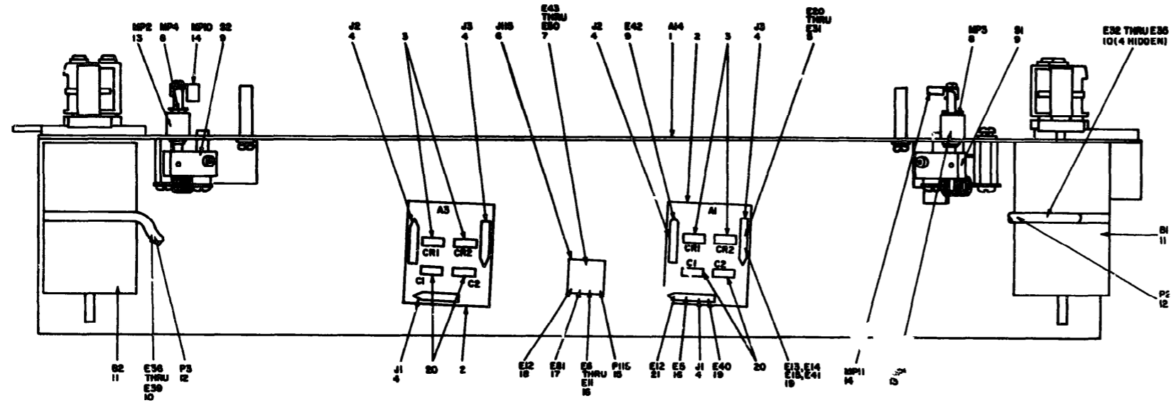
Figure 28 . Ribbon drive mechanism. 445411-1P parts location
