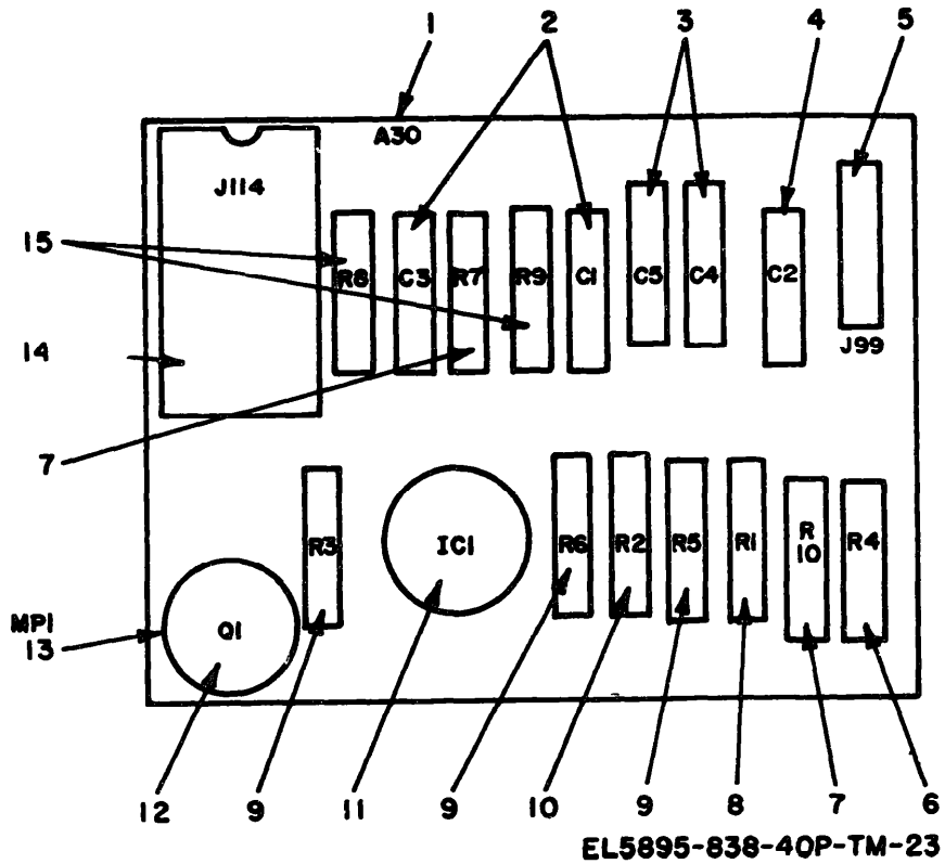
Figure 30. Magnetic pickup preamp subassembly 444470-1H, parts location
