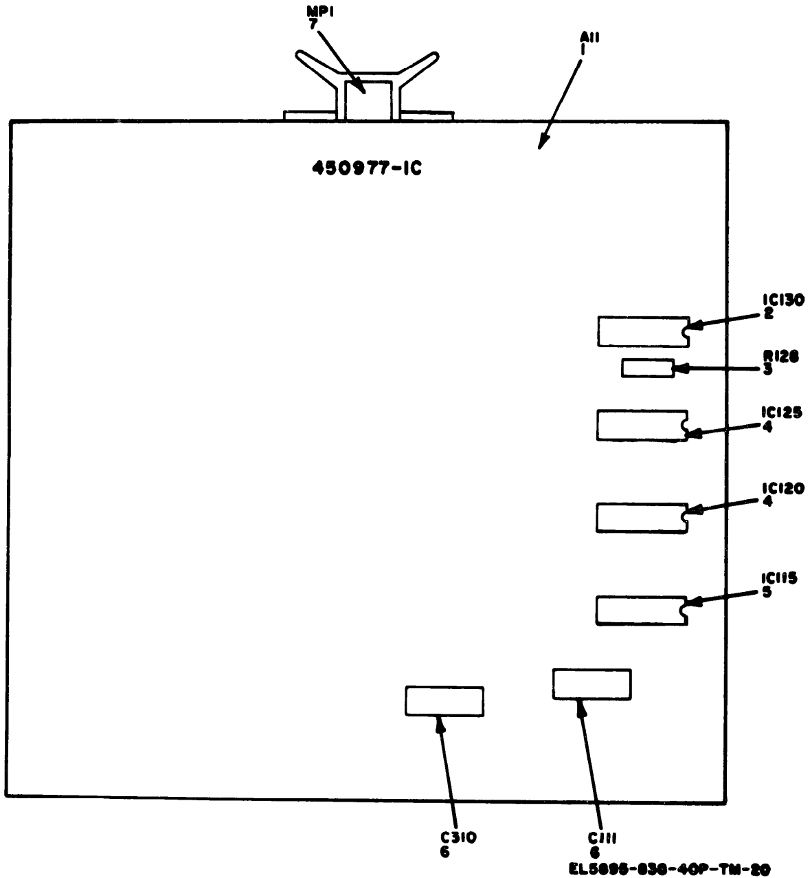
Figure 20. Circuit card assembly 450977-IC (ROM additions). parts location
