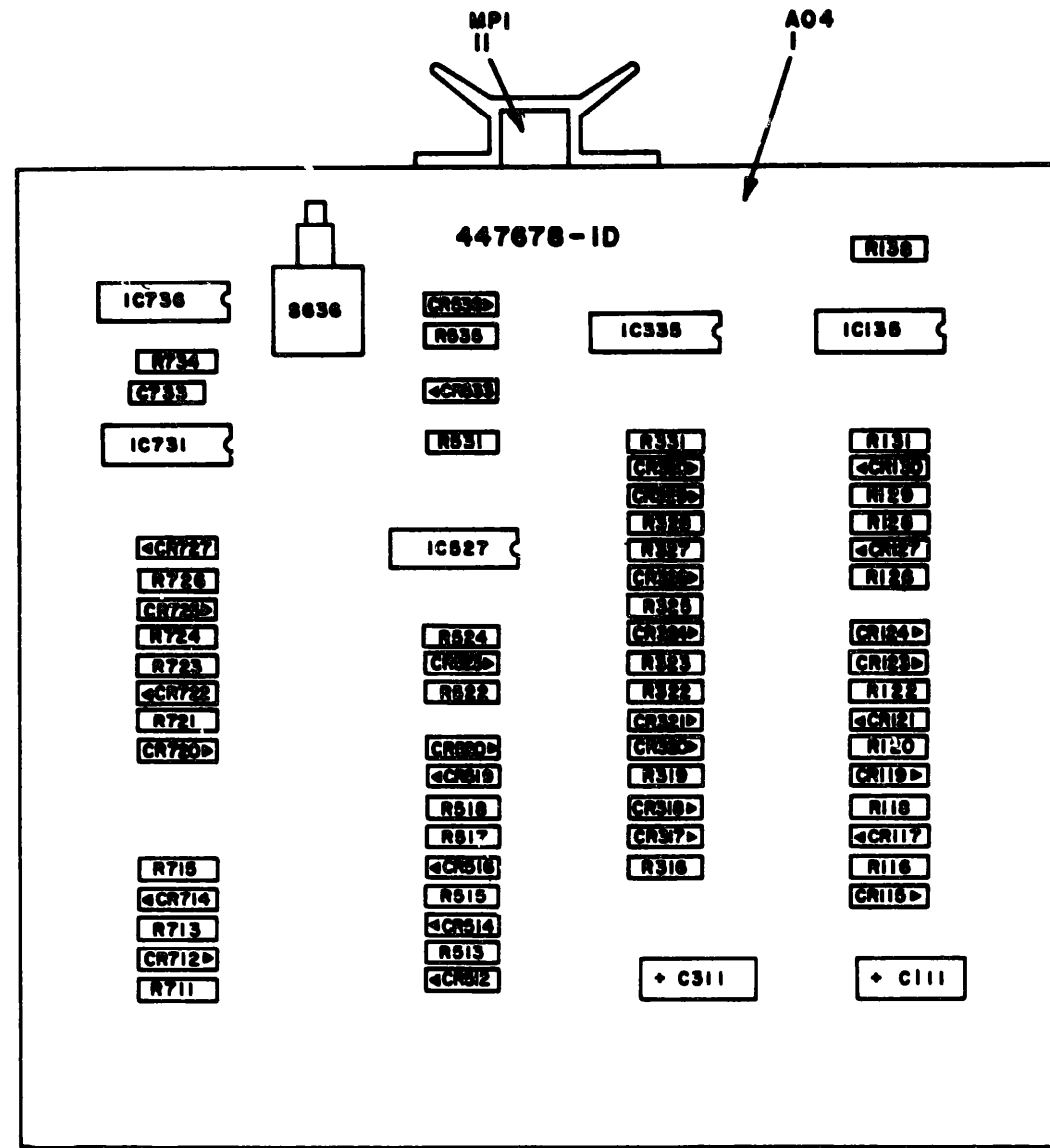
Figure 14. Circuit card assembly 447678-001D (line receiver module assembly) parts location
