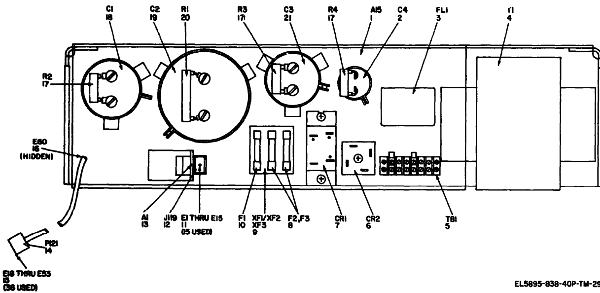
Figure 29. Power supply, 445300-1J, parts location
