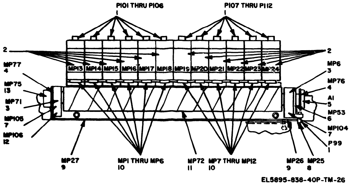
Figure 26. Helix assembly and hammer bank parts location
