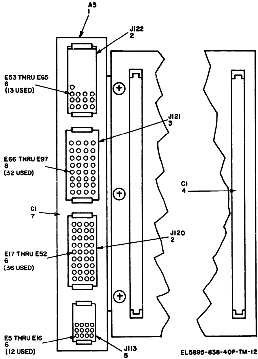
Figure 12. Card cage assembly. 445231-2W. parts location
