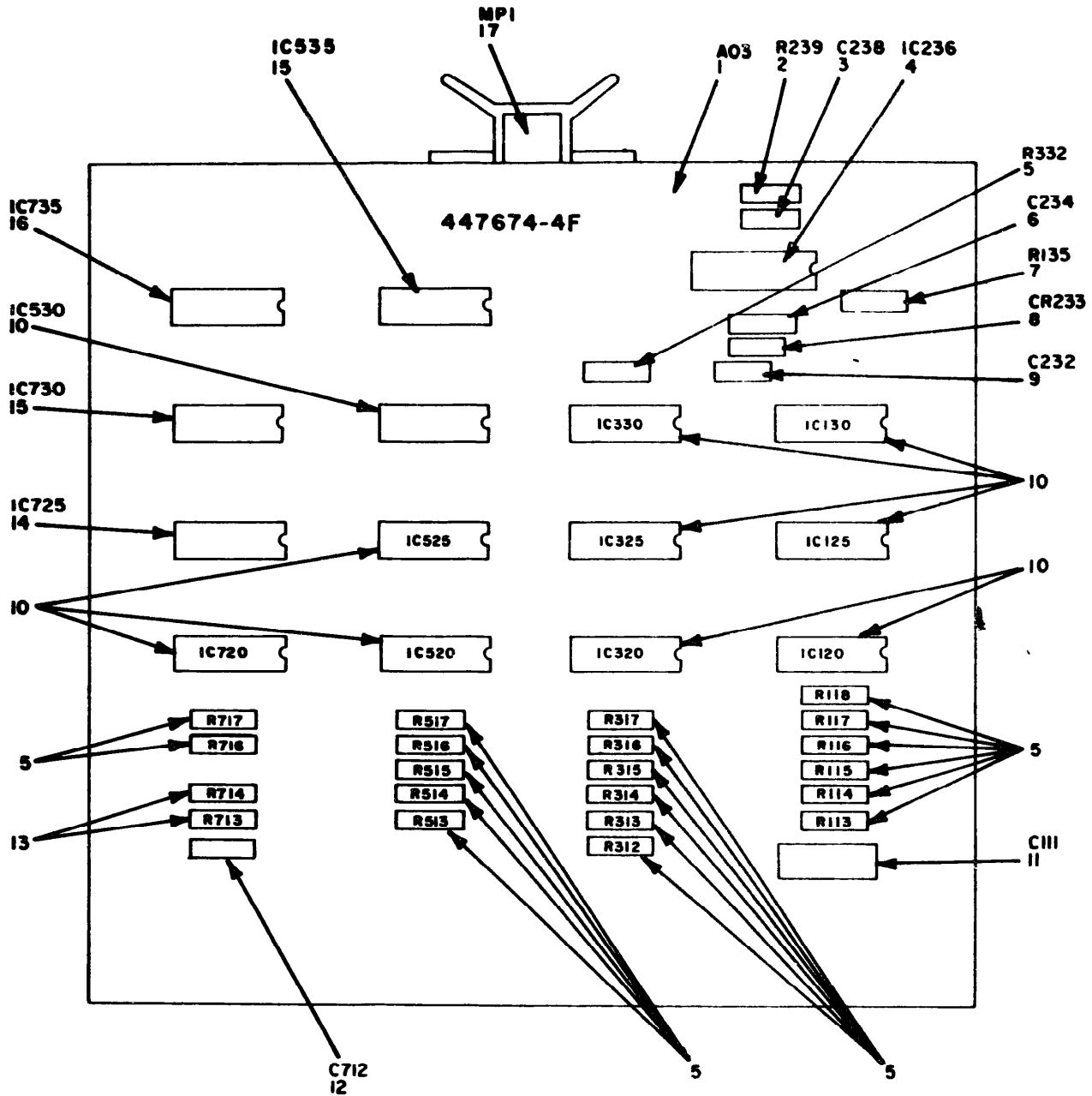
Figure 13. Circuit card assembly 447674 4F (line driver module assembly) parts location
