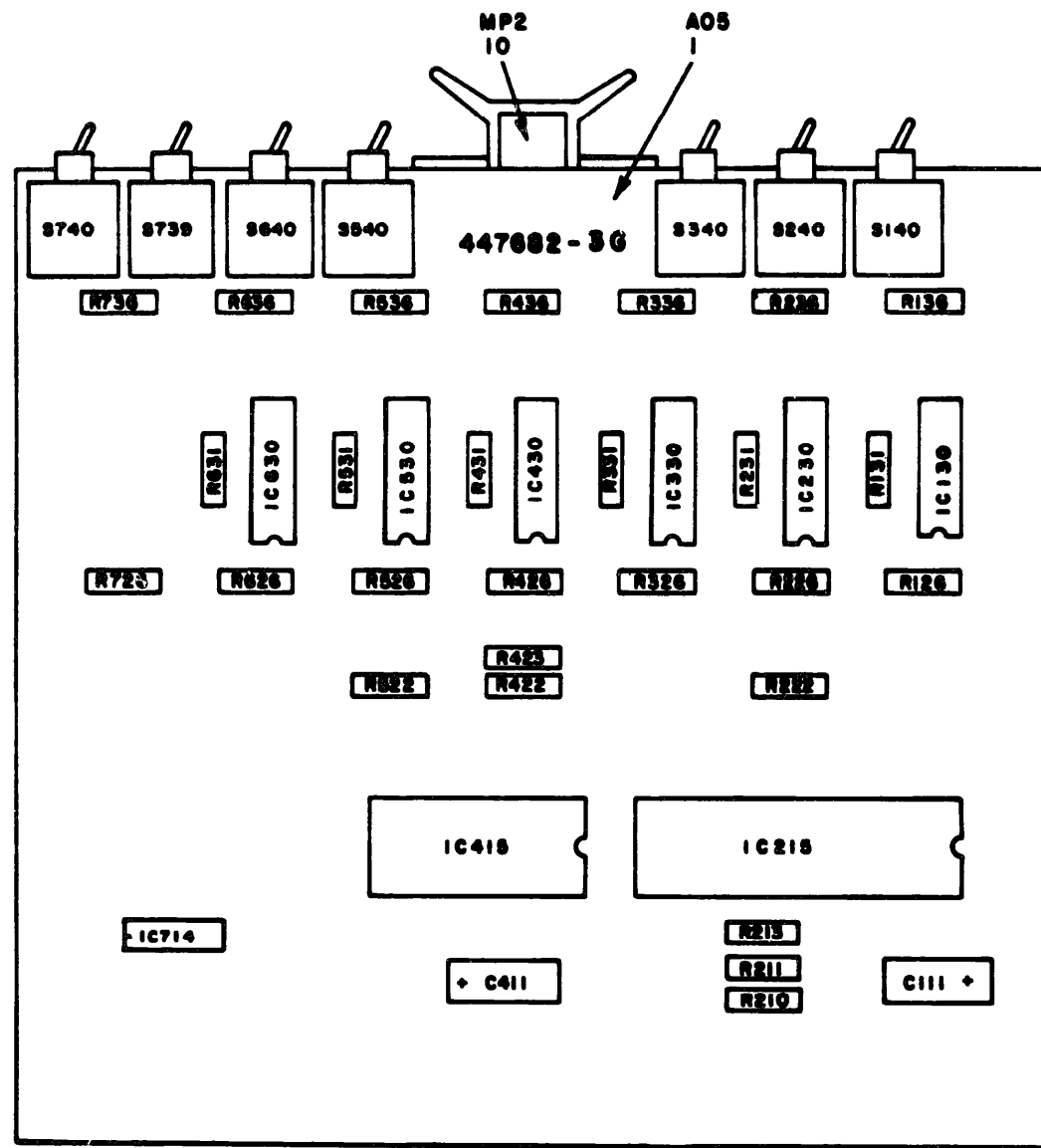
Figure 15 . Circuit card assembly, 447682-003G (shift register and print control), parts location
