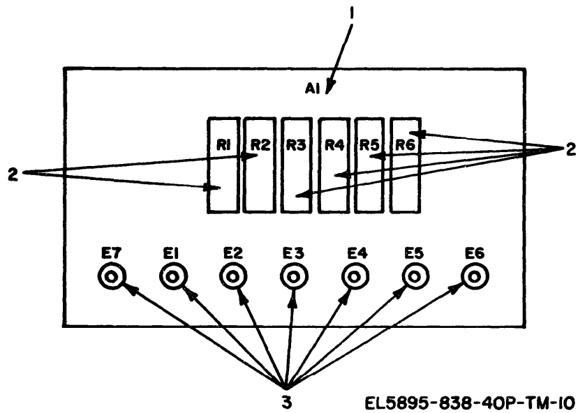
Figure 10. Circuit card assembly 445234-1A (resistor board), parts location
