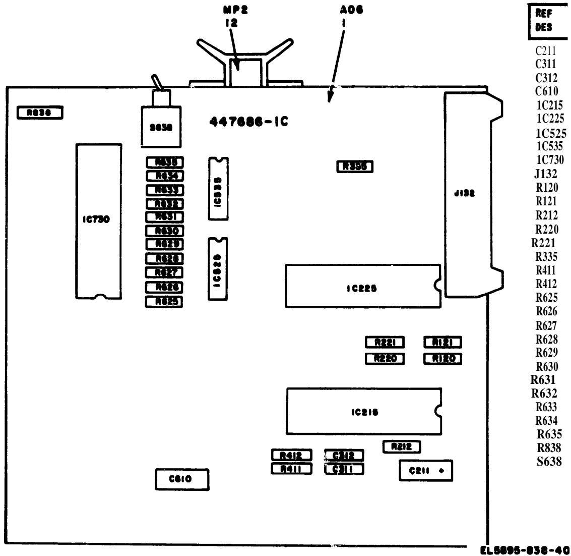
Figure 16. Circuit card assembly, 447688-1C (paper and hammer logic control), parts location
